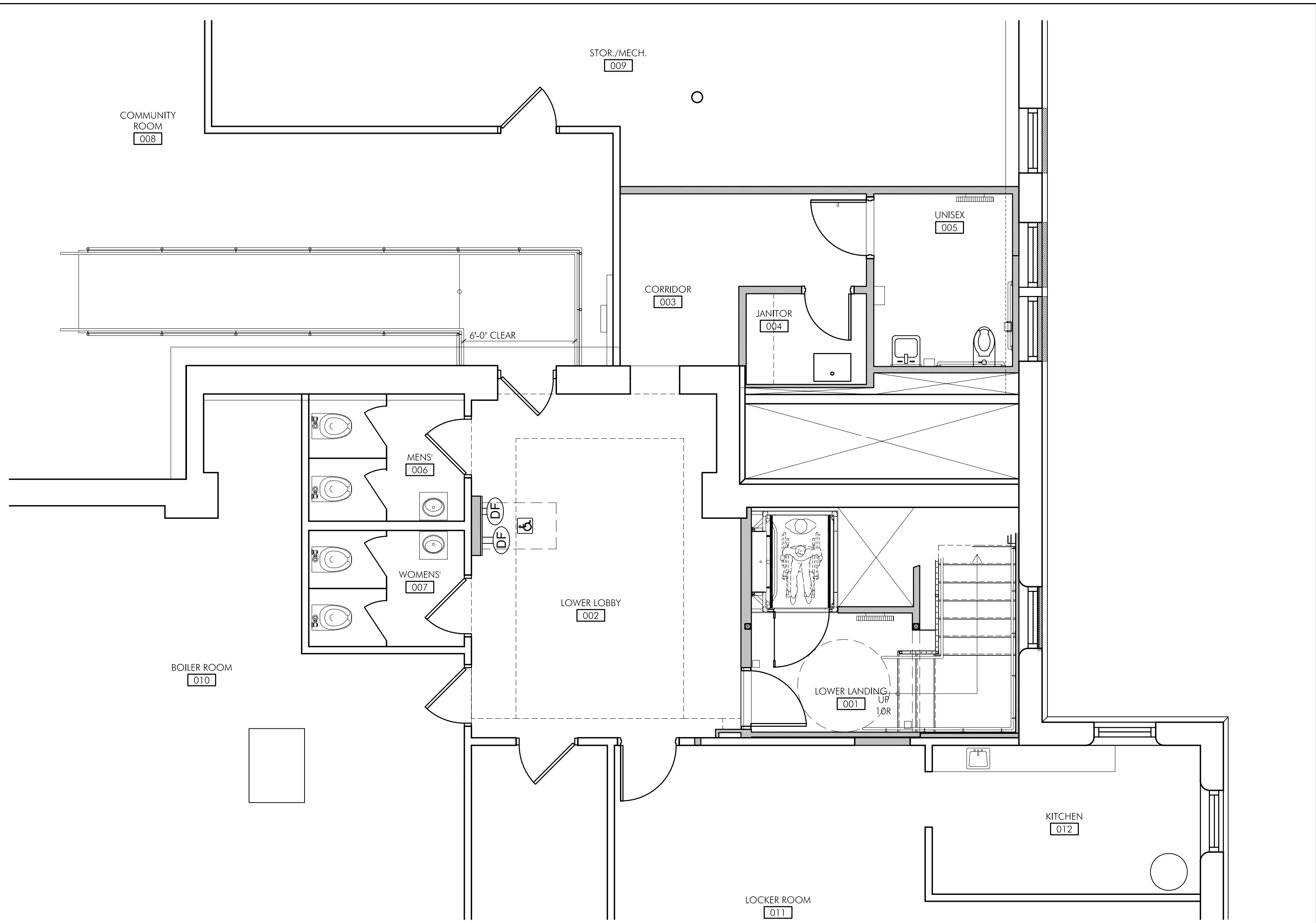
2 PARTIAL BASEMENT FLOOR PLAN SCALE: 1/4"=1'-0"
